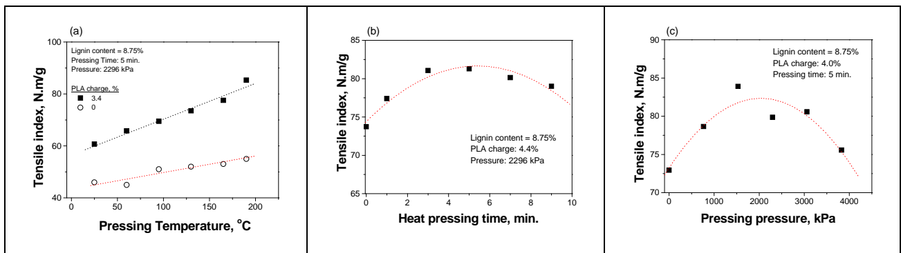
Figure 2. Characterization of press temperature, pressure, and press time on the strength properties of SW kraft linerboard with varying levels of PLA.
