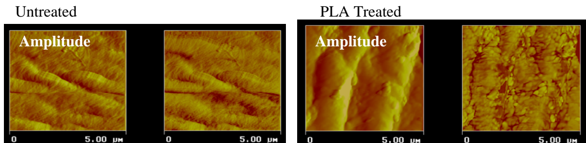
Figure 3. Amplitude and phase AFM analysis of SW kraft linerboard with 0.0 and 2.5% PLA applied and hot pressed (Press Conditions: 130 °C, 2.30 x 10 3 kPa, 5 min.).
